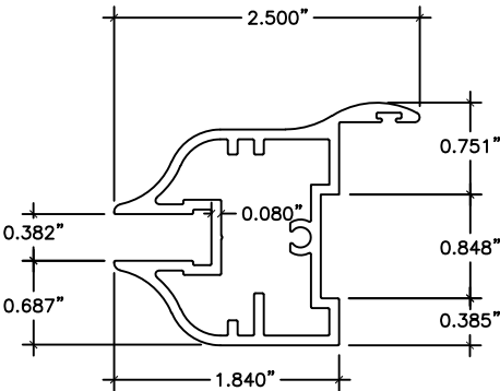
3B SASH PERIMETER 5/16" GLASS
